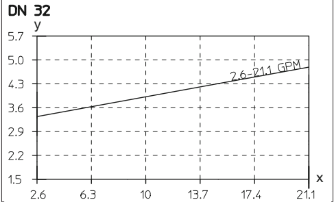
Illustr. 13: Min. differential pressures
