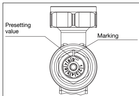
Illustr. 4 Presetting
