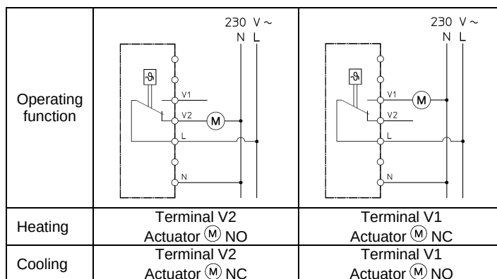
Illustr. 6.1 Wiring diagram Heating/Cooling
