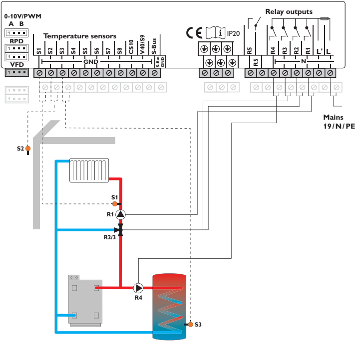
Scheme 4: 1 mixed heating circuit with DHW heating
