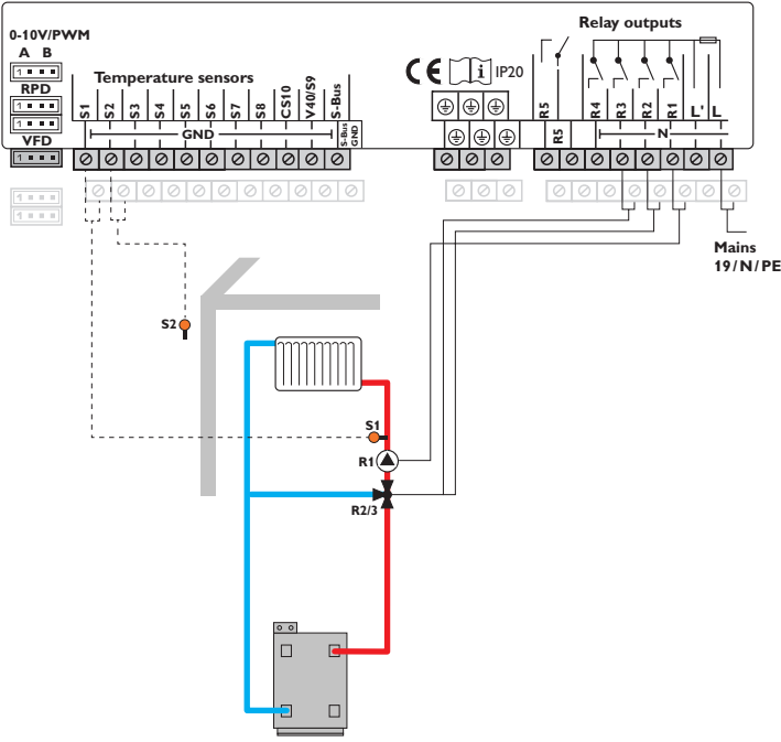
Scheme 1: 1 mixed heating circuit
