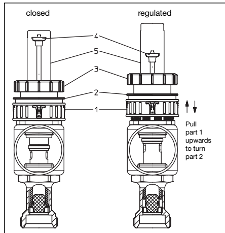
Illustr. 7.1: Setting of flow measuring and regulating devices
