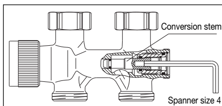
Illustr. 8 Conversion to one pipe operation
