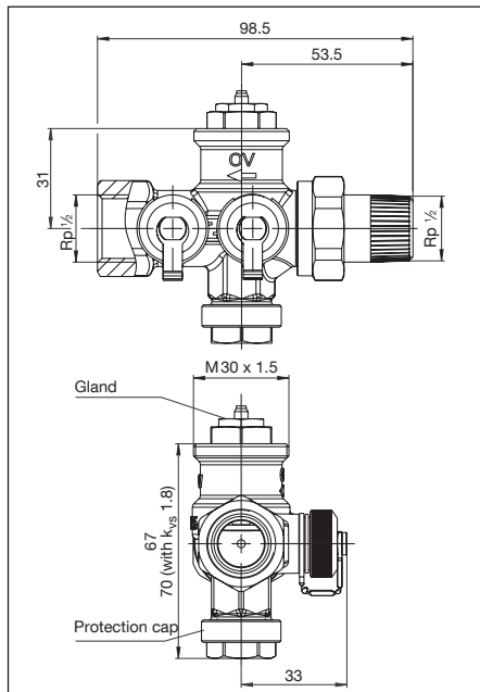
Illustr. 4.2 Dimensions
