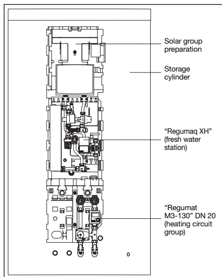
Illustr. 19 Summary of components
