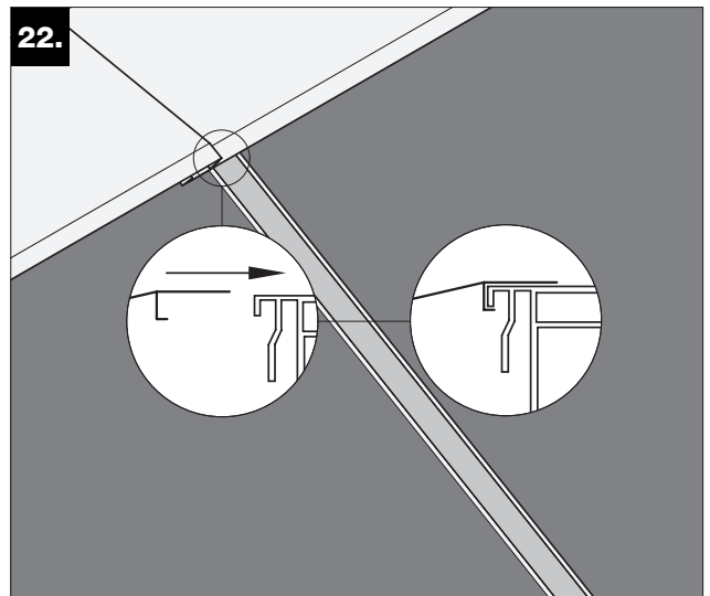
22. Position upper metal closing sheet so as to fit groove into the collector rebate.
