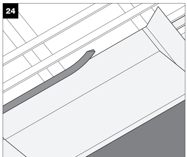
24. Bond black foam rubber sealing tape onto the upper metal cover sheets along the groove.
