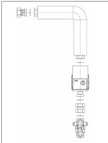
Illustr. 1.4 Circulation connection set with pump Wilo-Yonos PARA Z 15/70 RKC and adapter
