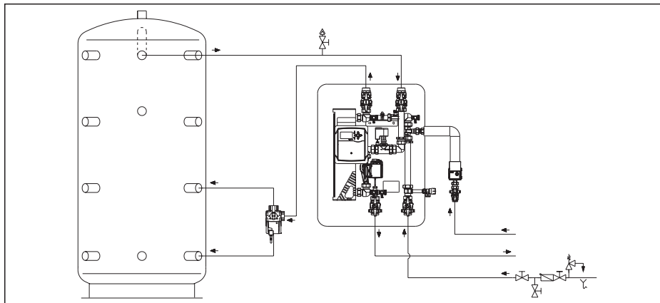
Illustr. 1.6 Connection example
