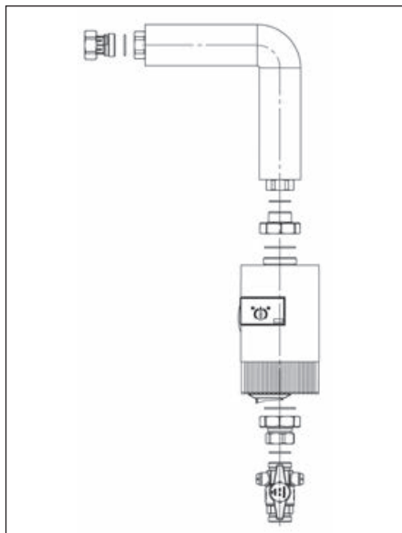
Illustr. 1.5 Circulation connection set with pump Wilo Stratos PARA Z 25/1-12 RK and adapters
