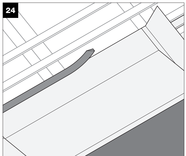
Bond black foam rubber sealing tape onto the upper metal cover sheets along the groove.
