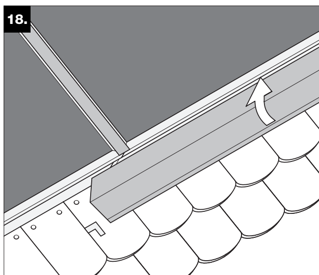
18. Fit in lower metal sheets for roof covering.
