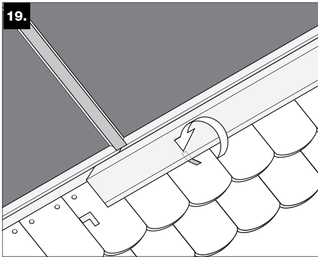
Fix lower metal sheets for roof covering with sheet metal clamps.
