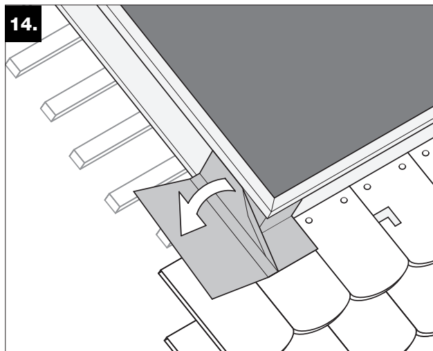
14. Push down the upright metal side until flush with roofing.
