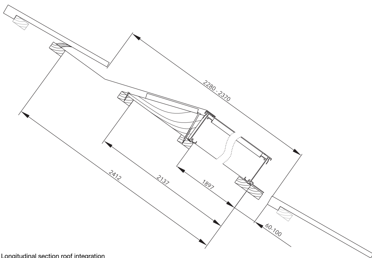
Longitudinal section roof integration
