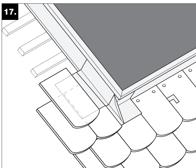
17. Cover each metal sheet with a tile.
