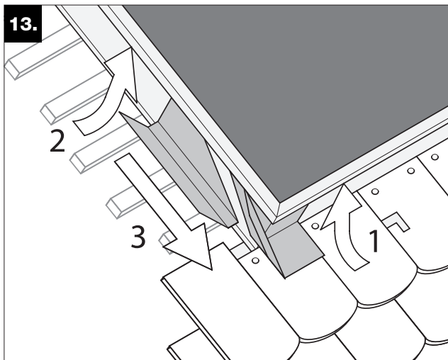
13. Introduce both pieces of the gusset into the lower collector groove (1 + 2) and push together (3).
