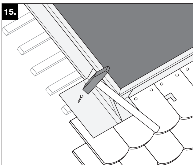
15. Fix individual metal side sheets onto the battens with clout nails.
