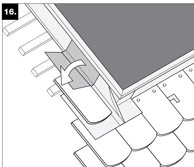
16. Insert metal sheets into the lower groove and align with the upper edge of the upper batten. Starting from the bottom to the top, mount metal sheets onto each neighbouring row of tiles with an overlap.
