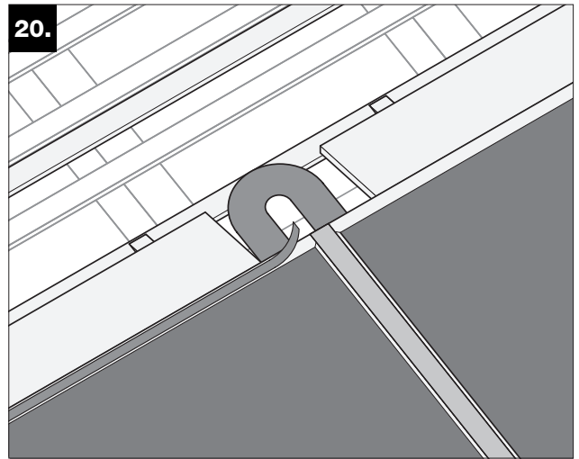
Bond cellular rubber sealing tape onto the upper collector edge.
