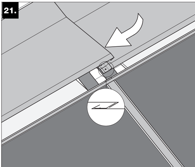
Link upper metal connection sheets with each other by interlocking them at the rebate points and fix with dorsal gusset plate.
