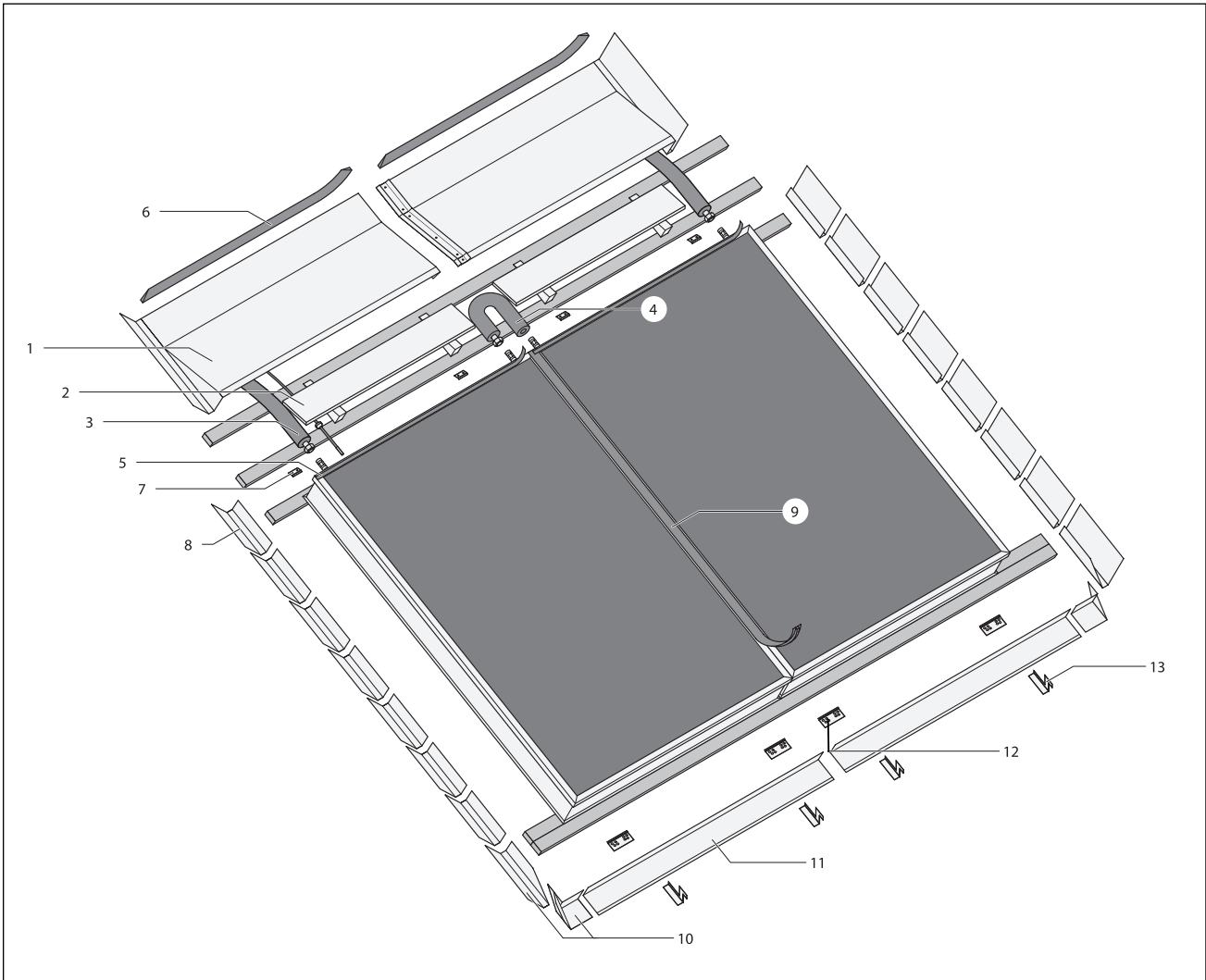
Basic set for roof integration, item no. 136 12 93 (collectors are not included)
