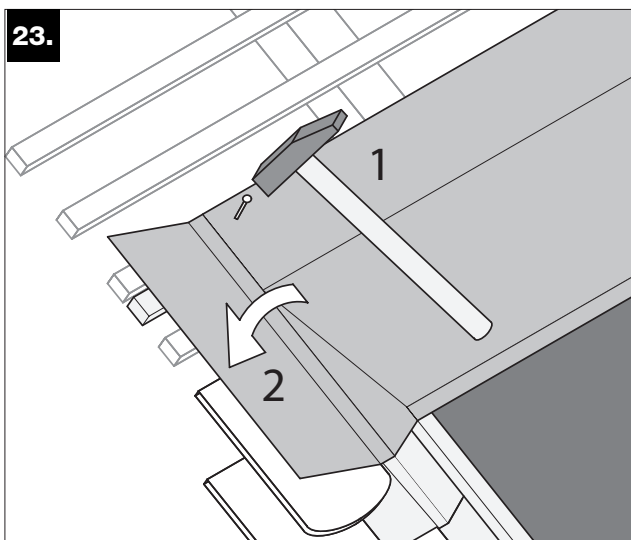
Nail upper metal closing sheets onto the battens and align the up-right metal side.
