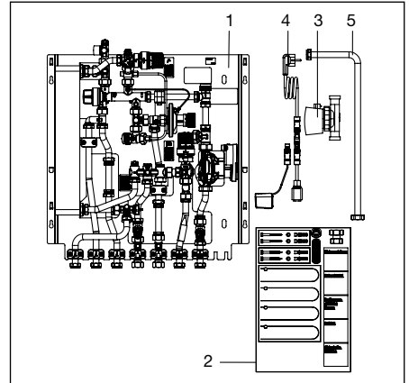
Fig. 3.1 Fourniture
