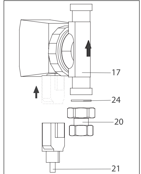
Illustr. 6.2 Pump orientation
