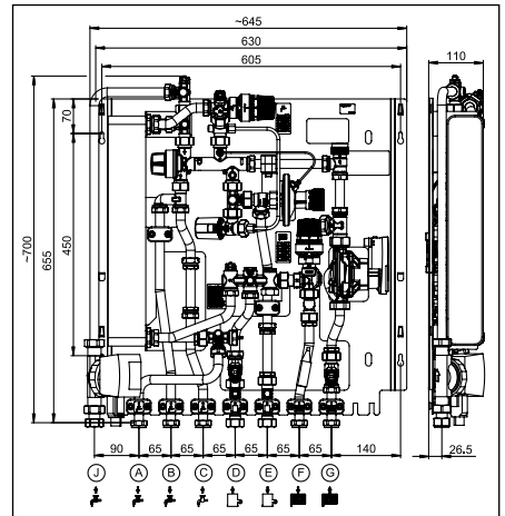
Illustr. 4.3 Dimensions with constant temperature circuit and circulation pipe
