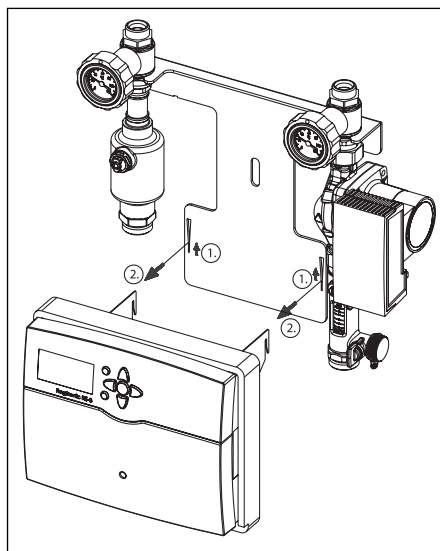
Illustr. 16 Separation of controller
