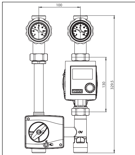
Illustr. 28 Dimensions "Regumat M3-130" DN 20
