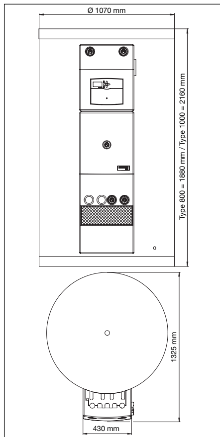
Illustr. 2 Dimensions
