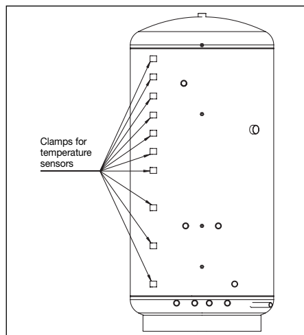
Illustr. 6 Storage cylinder with dismantled insulation
