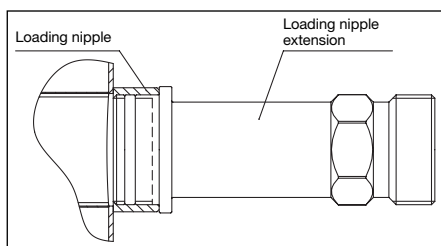
Illustr. 5 Mounted extension for loading nipple
