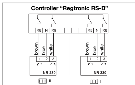
Illustr. 27 Controller
