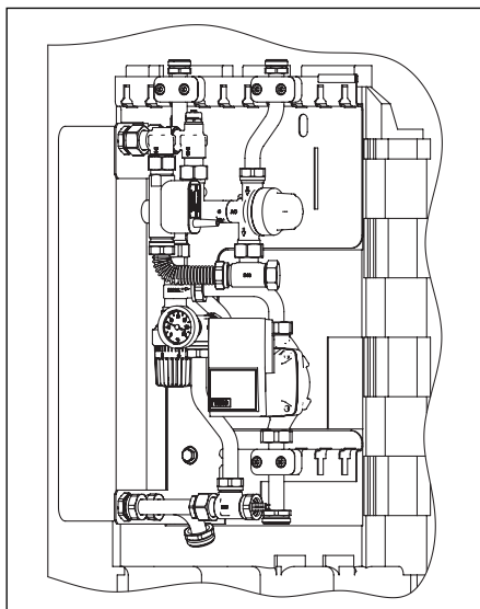
Illustr. 13 Installation of fresh water station
