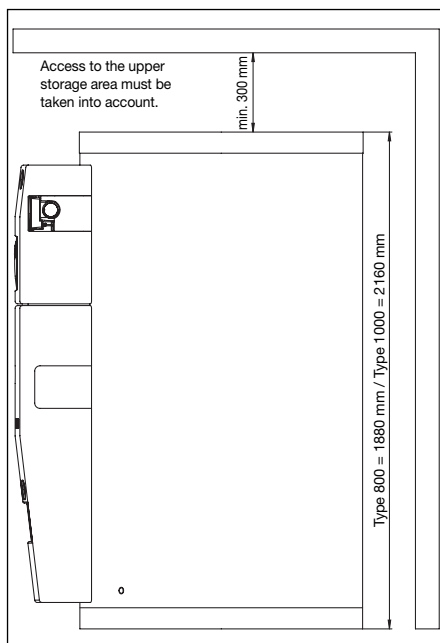
Illustr. 4 Installation dimensions
