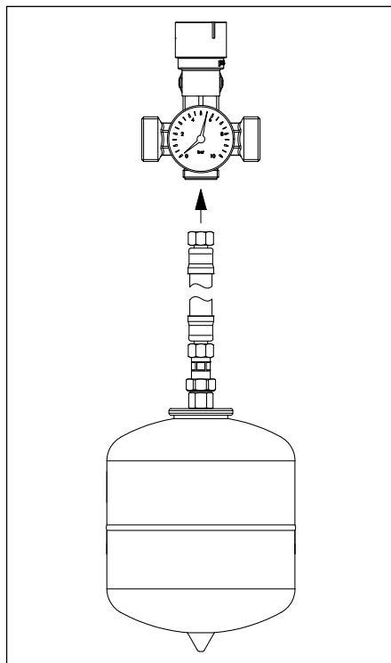
Connection of the expansion tank
