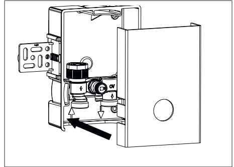
Illust. 8: Fitting of the protection cover
