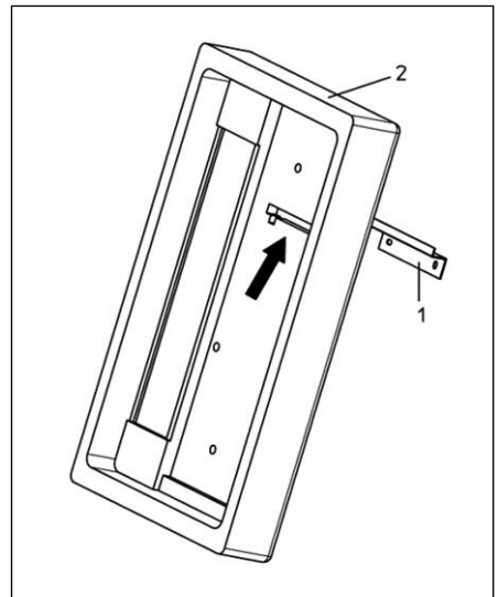
Illustr. 17: Rear insulation shell, angled wall bracket
