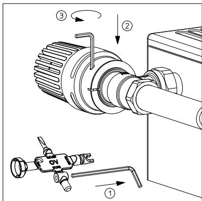
Montage/Demontage Thermostat „Uni LHB” Installation/removal thermostat “Uni LHB” Montage/démontage thermostat «Uni LHB»
