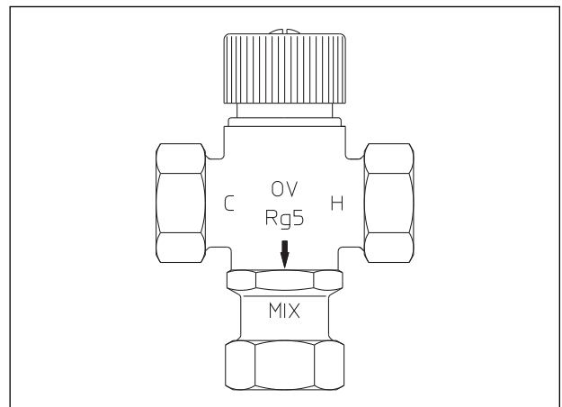
Illustr. 8: Thermostatic mixing valve "Brawa-Mix", OV item no. 130 03 51 or 130 03 52
