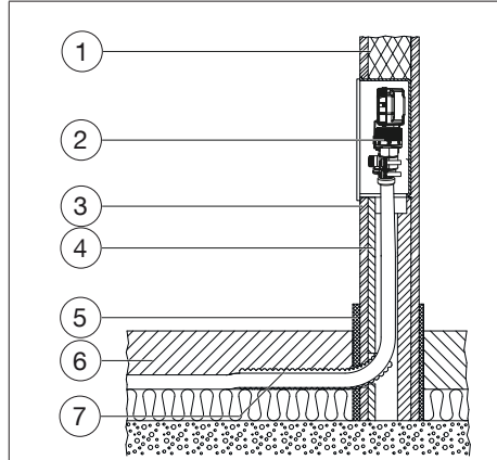
Illust. 7: Installation cross section
