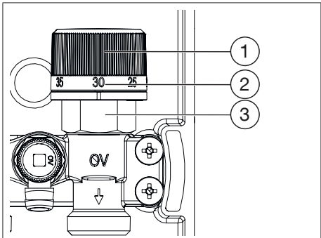
Illust. 4: Handwheel
