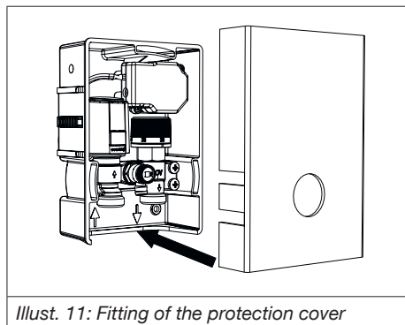
Illust. 11: Fitting of the protection cover
