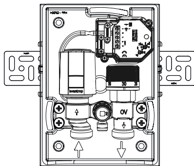
Illust. 9: "Unibox T-RTL R-Tronic" with brackets
