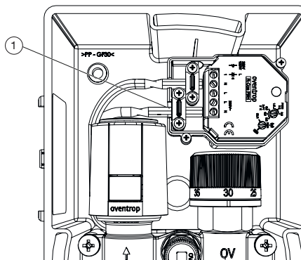
Illust. 10: Electrical connection of the wireless receiver "R-CON FBH"
