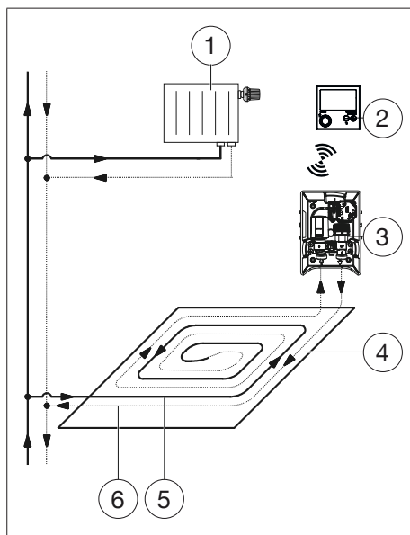
Illust. 8: Connection
