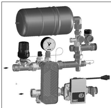
Illustr. 1.1 “Regufloor HX” Control unit
