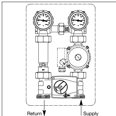
Installation example "Regumat M4"
