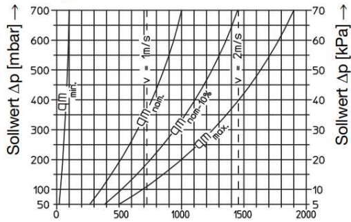
DN 20: kvs = 5,0
