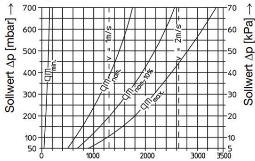
DN 25: kvs = 7,5
