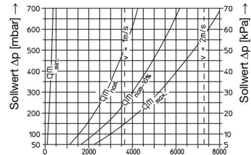
DN 32: kvs = 10,0
