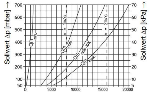
DN 50: kvs = 34,0
