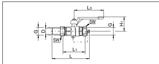
Item no. 106 65 04-10 (DN 15 to DN 32) Aluminium lever
