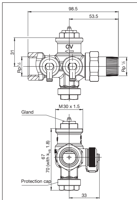
Illustr. 4.2 Dimensions
