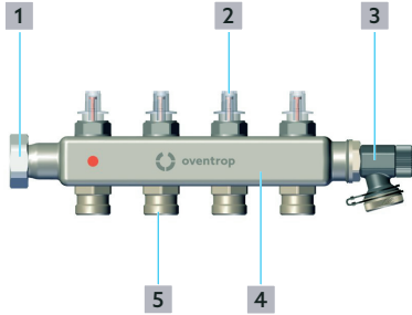
Fig. 2: Construction of the distributor for the flow indicator
