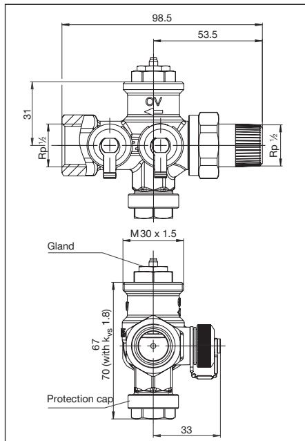
Illustr. 4.2 Dimensions
