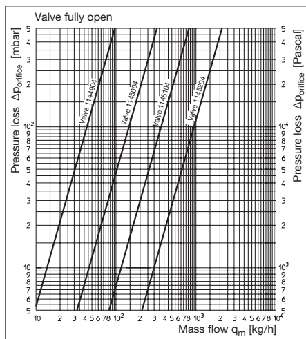
Chart 4.1 Flow rate depending on the pressure loss ( \Delta p_{\text{orifice}} ) via the pressure test points (see illustr. 4.1)
