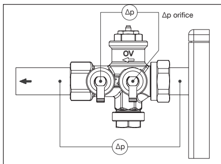
Illustr. 4.1 Differential pressure measurement
