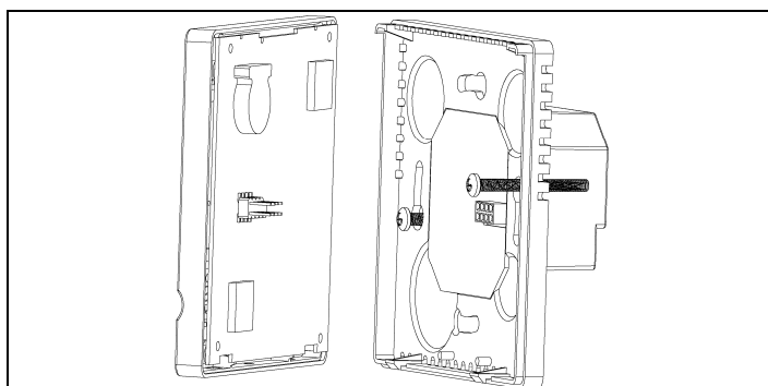
Illustr. 6.1 Installation of the thermostat
