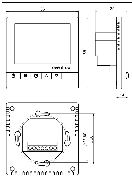
Illustr. 4.1 Dimensions
