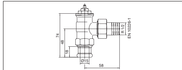
Dimensions of angle pattern valve
