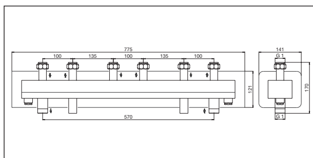
Dimensioni “HydroFixx” DN 20, 3 circuiti
