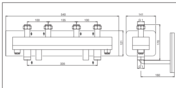
Dimensioni “HydroFixx” DN 20, 2 circuiti
