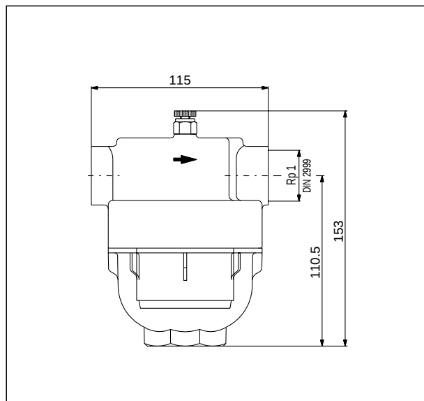
"Aquanova Compact" Item no. 612 05 08 (DN 25), brass
