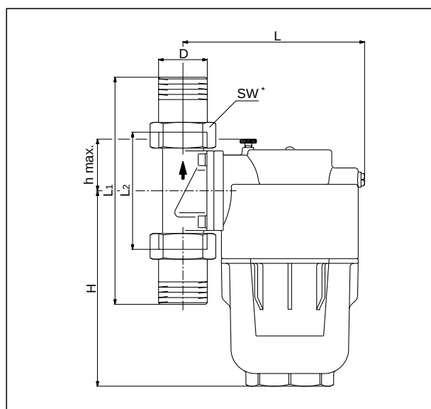
"Aquanova Compact E" Item no's. 612 07 06-10 (DN 20 – DN 32)
