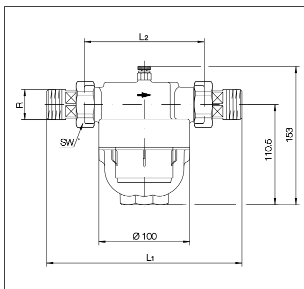
"Aquanova Compact" Item no's. 612 25 06-10 (DN 20 – DN 32), bronze
