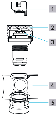
Fig. 3: Design of the QM valve insert
