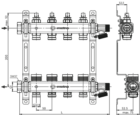
Fig. 6: Dimensions
