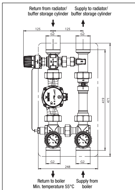
Illustr. 4.6 "Regumat RTA-180" DN32 with standard insulation Supply on right hand side Boiler is located below the "Regumat"
