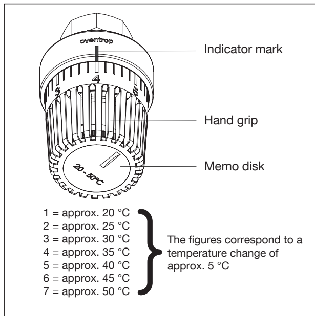
Temperature controller - Heating circuit
