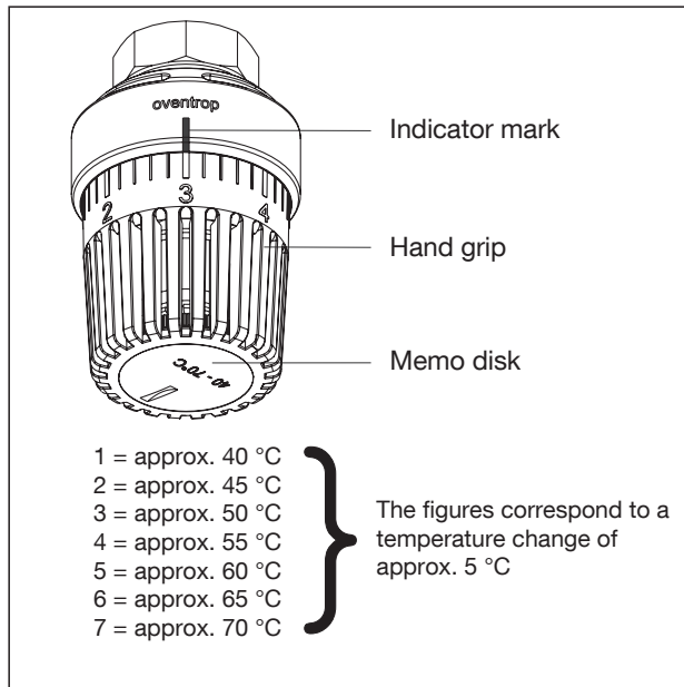
Temperature controller - Potable water
