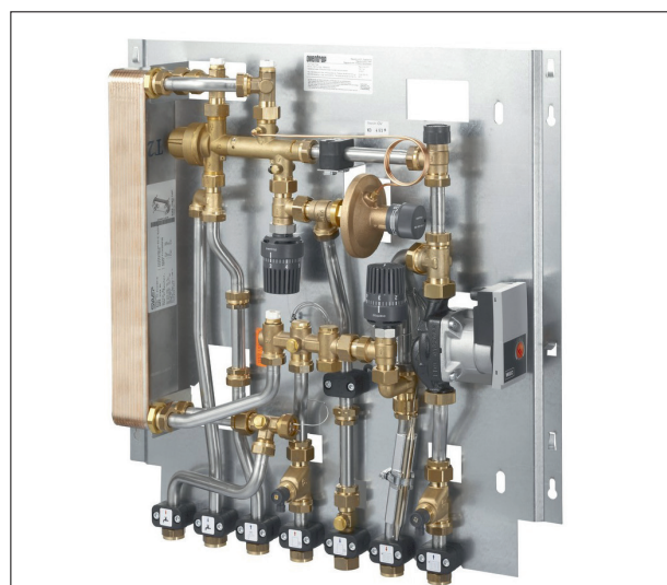
“Regudis W-HTF” - variable temperature heating circuit
