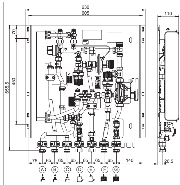
Dimensions with variable temperature heating circuit
