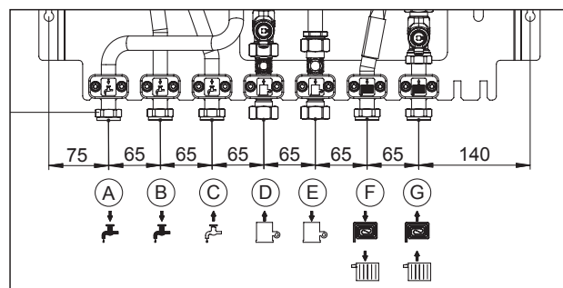
Dimensions with variable temperature heating circuit
