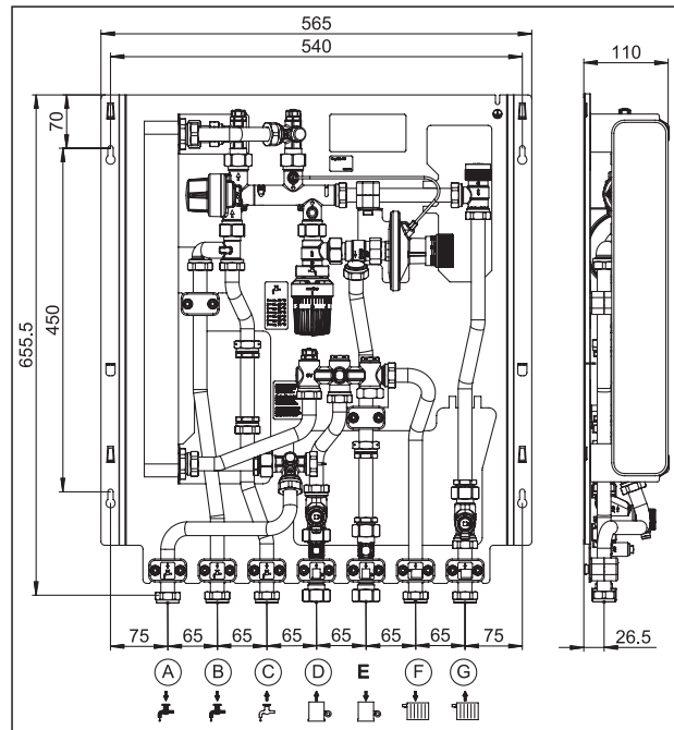
Dimensions with constant temperature heating circuit
