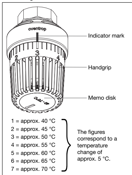
Illustr. 8.3 Setting potable water temperature
