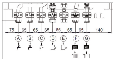
Illustr. 4.3 Connection sizes
