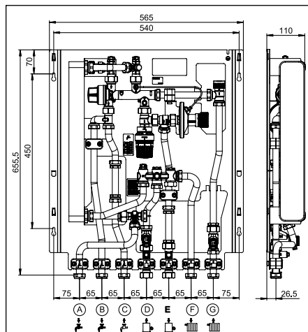
Illustr. 4.2 Dimensions with constant temperature circuit
