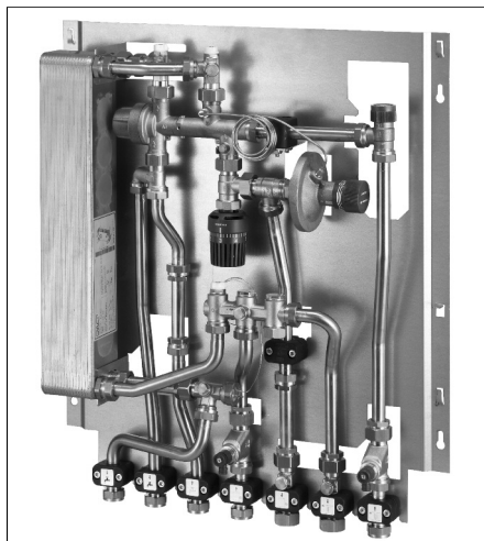
Illustr. 1.1 "Regudis W-HTF" dwelling station
