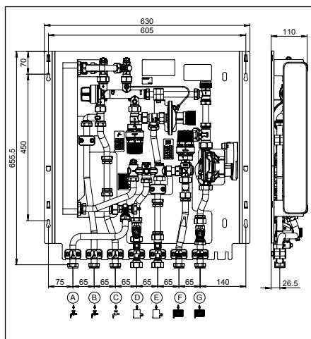
Illustr. 4.4 Dimensions with variable temperature circuit
