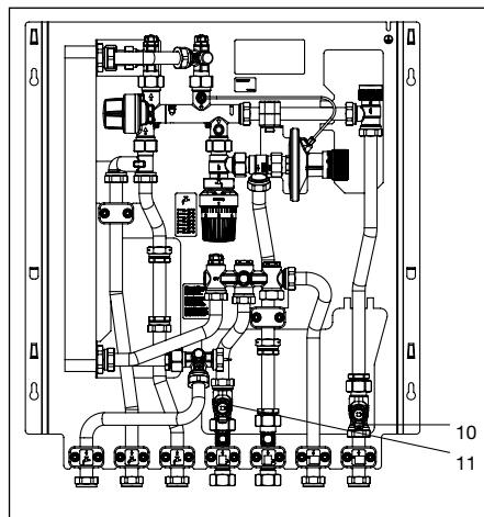
Illustr. 8.1 Installation position of strainers
