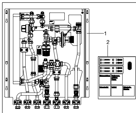
Illustr. 3.1 Fourniture
