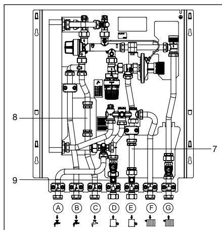
Illustr. 6.1 Installation cold water meter and heat meter
