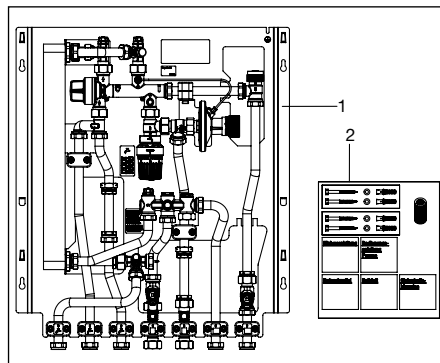
Illustr. 3.1 Extent of supply
