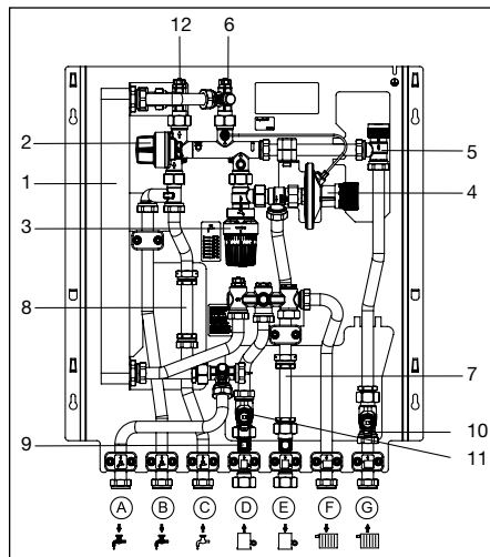
Illustr. 5.1 Construction with constant temperature circuit
