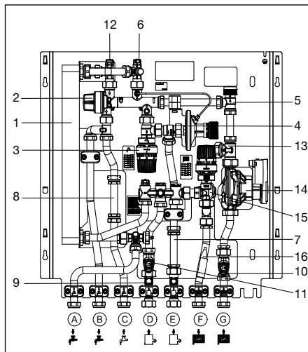
Illustr. 5.2 Construction with variable temperature circuit
