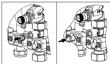
Illustr. 6.2 Installation sensor for heat meter
