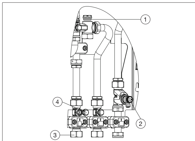
Illust. 2: Removal of the plugs Regudis W-HTU/TU and Regudis W-HTF
