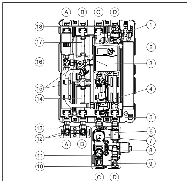
Illust. 2: Construction of the Regudis H-MT
