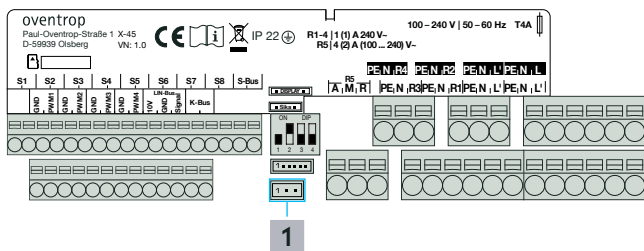
Fig. 10: Connecting block Regumaq X-45
