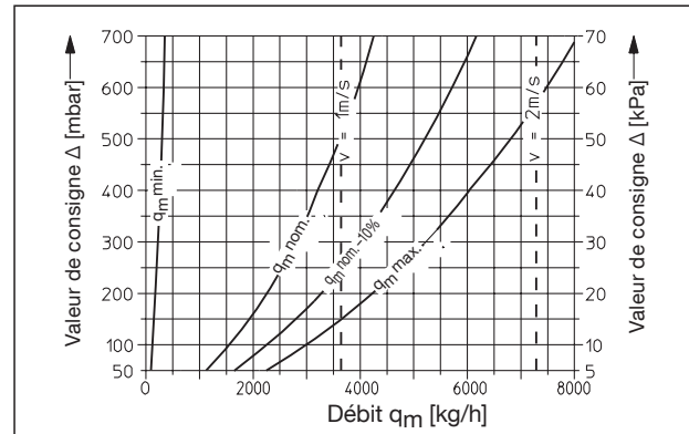
DN 32 : k_{VS} = 10.0
