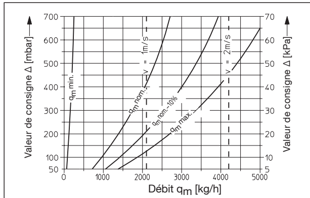
DN 25 : k_{VS} = 7.5
