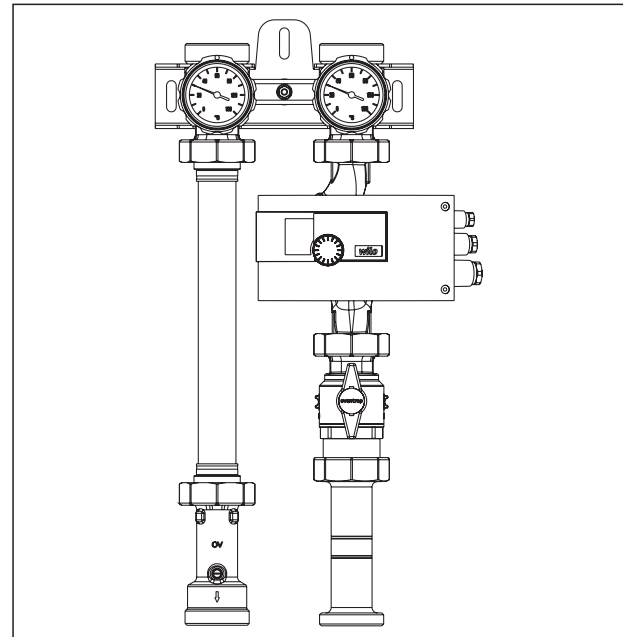
Regumat S-180 plus DN 32 with pump ball valve
