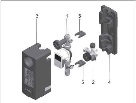
Abb. 6.4 Pumpenstrang
