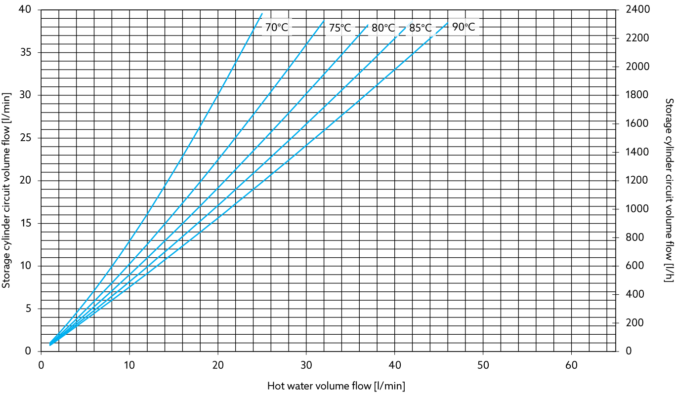
Volume flow of the storage cylinder circuit at different flow temperatures
