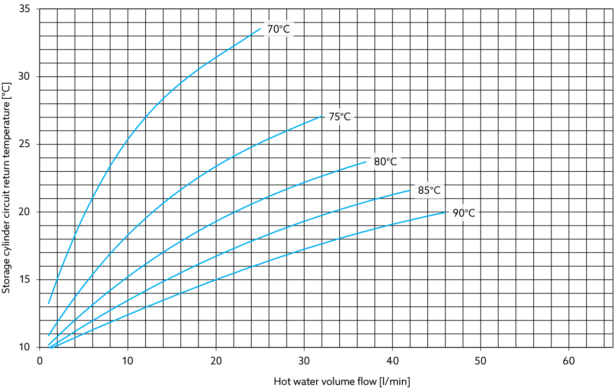
Return temperature of the storage cylinder circuit at different flow temperatures
