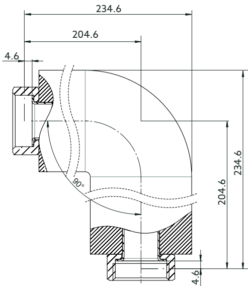
Fig. 5: Dimensions of the pipe elbow
