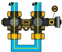
Normal operation
