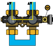
Bypass operation
