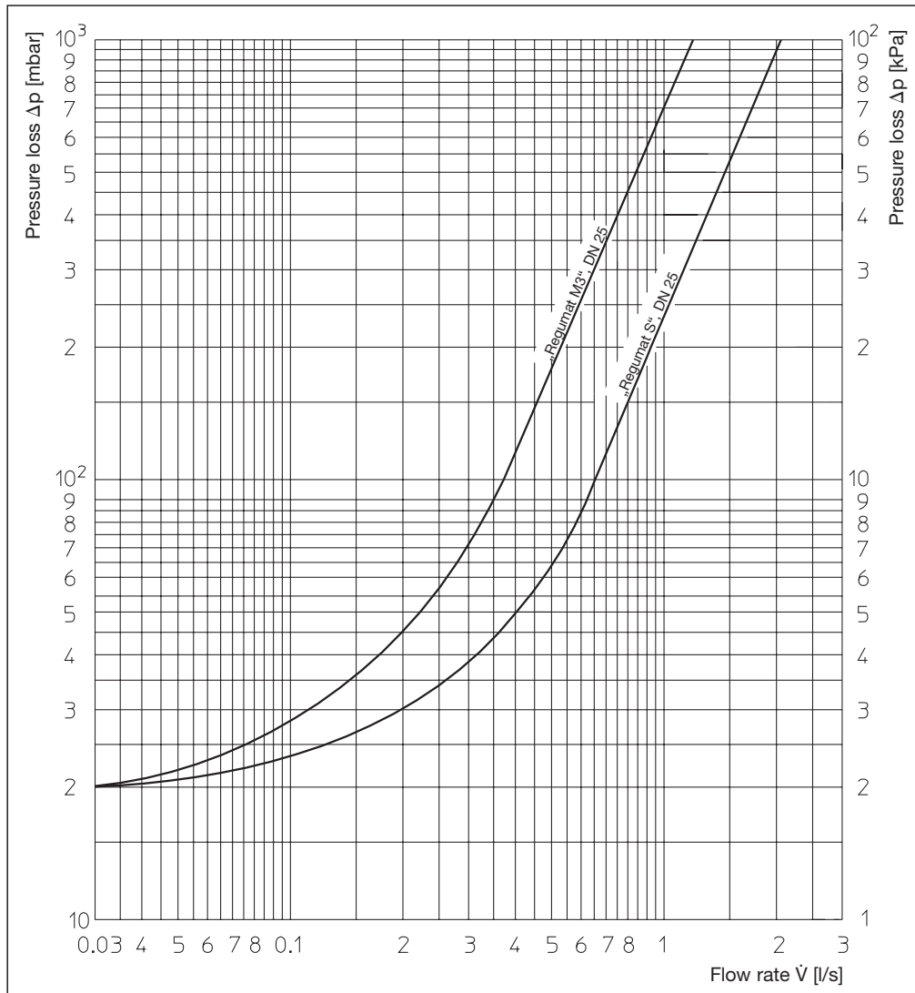
Flow chart Regumat-130 DN 25
