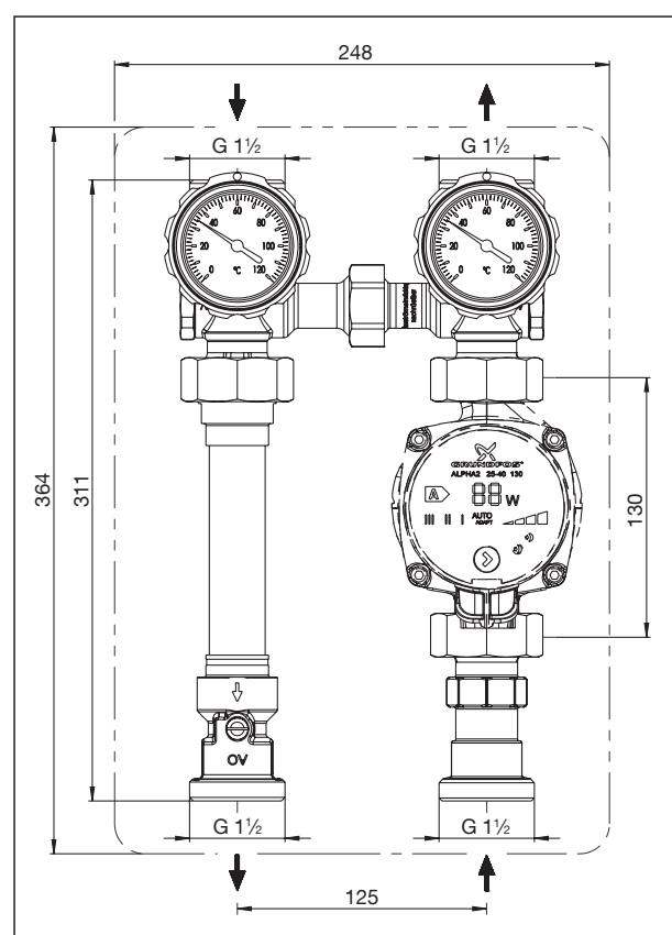
Dimensions Regumat S-130 DN 25
