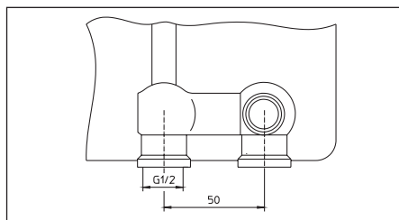
Abb. 8 Ventilgarnitur G \frac{1}{2} IG
