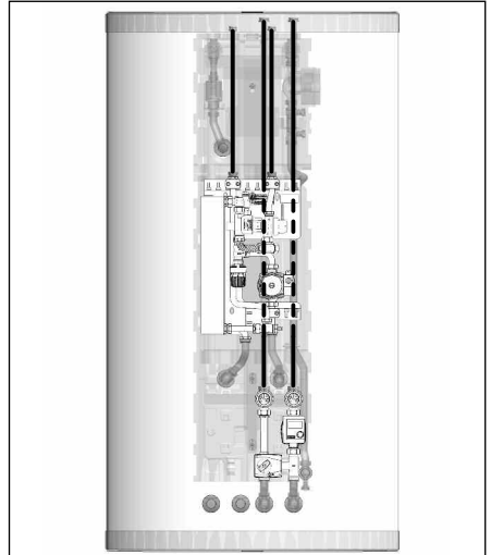
Illustr. 1.1 Installation scheme for connection set (Item no.: 138 35 80)
