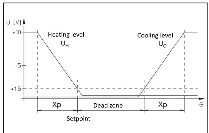
Function diagram
