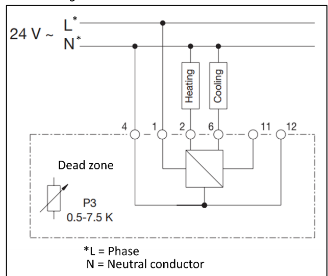
Wiring diagram
