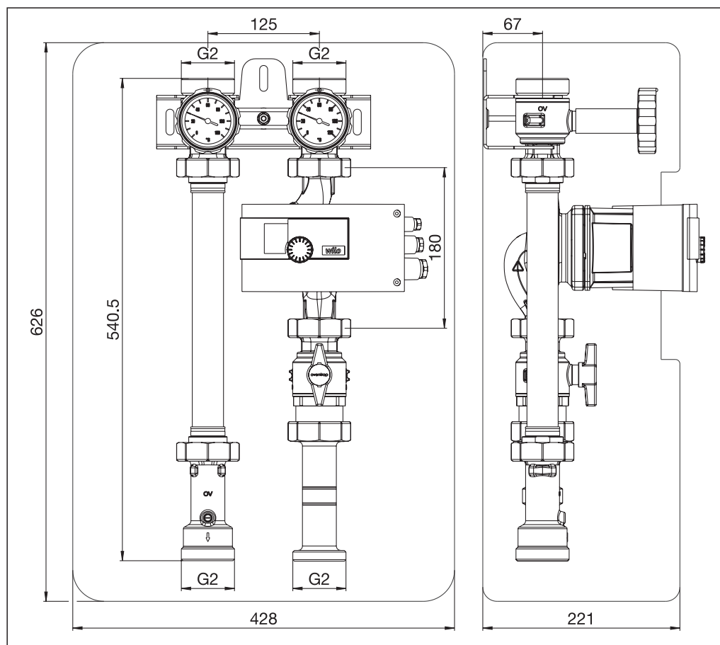
Encombresments Regumat S-180 plus DN 32
