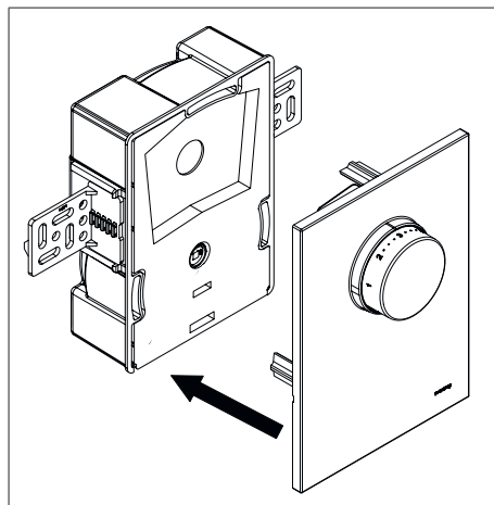
Illustr. 11: Positioning the cover plate with handwheel
