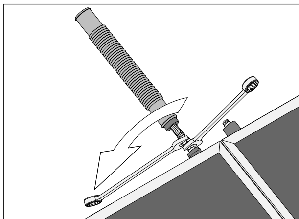
Illustr. 4 Tighten connection with \frac{1}{4} turn. Hold firm while tightening to avoid damage to the collector and coupling hose. !
