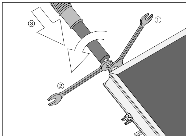
Illustr. 2 Hold collector hose connection firm while tightening to avoid damage to the collector connection and hose. Slide gaiter over insulation. !
